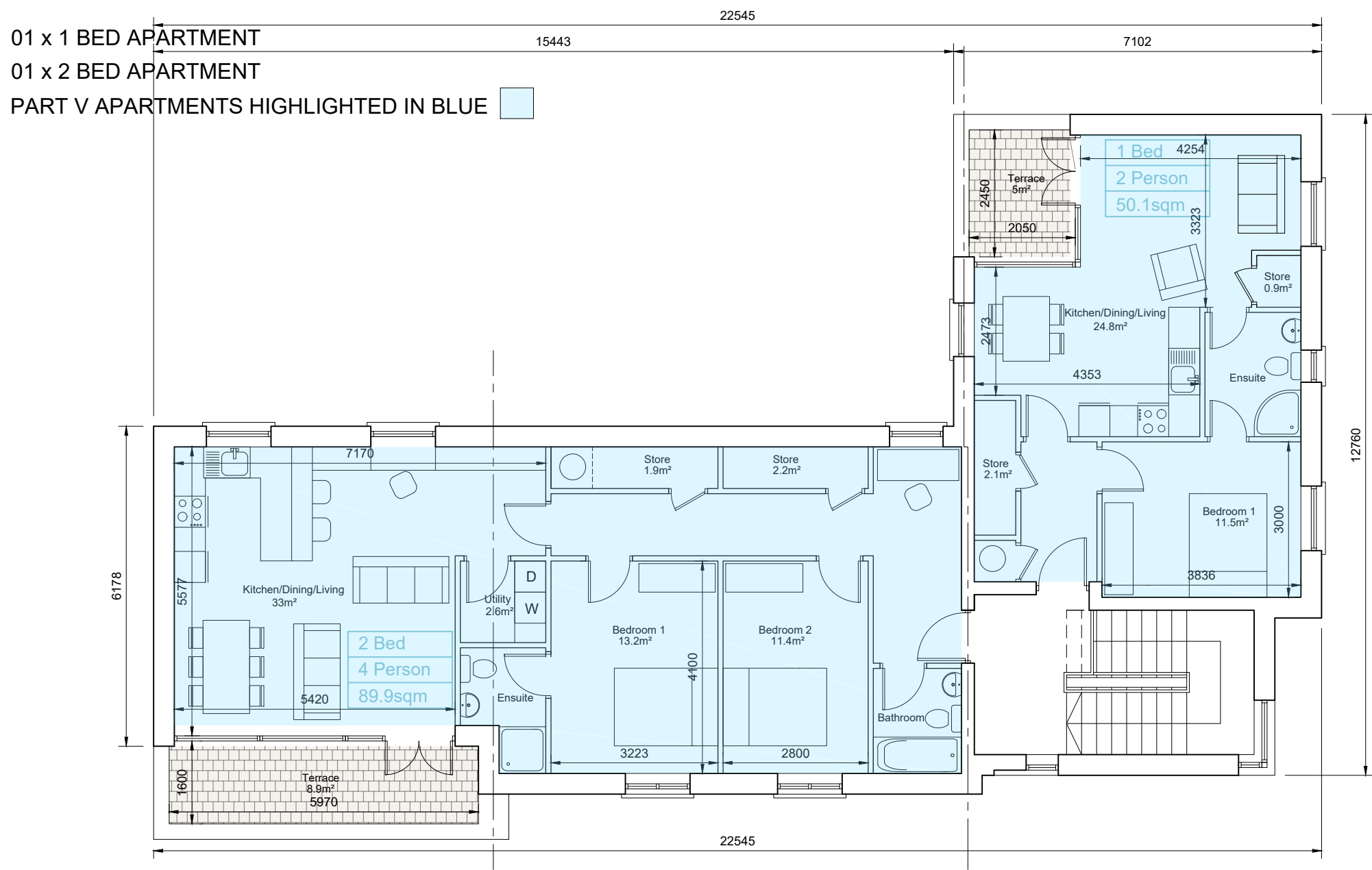
SECOND FLOOR PLAN Unit Nos 013-017
